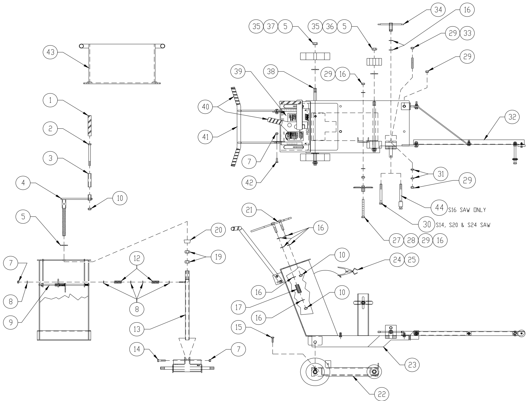
HydraCart Assembly
