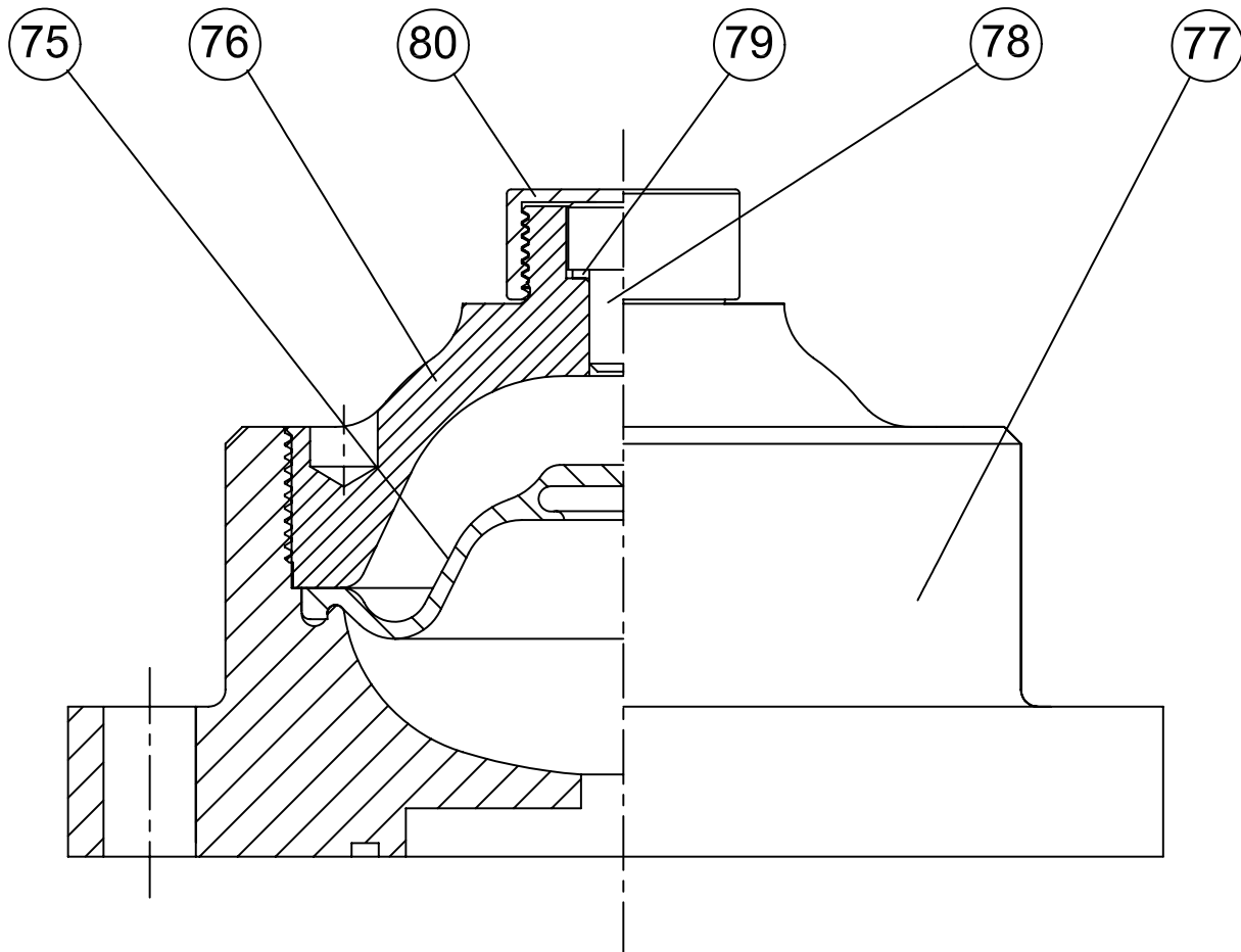
Figure 6-4. Accumulator Assembly
