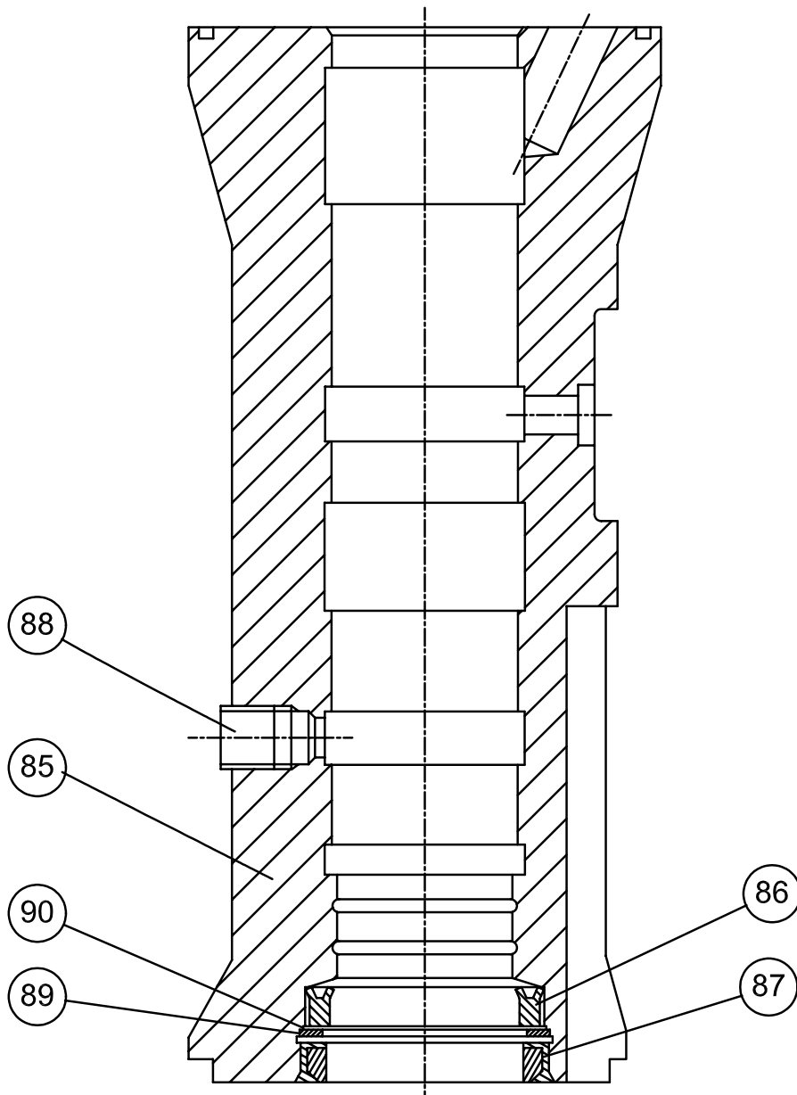
Figure 6-5. Cylinder Assembly
