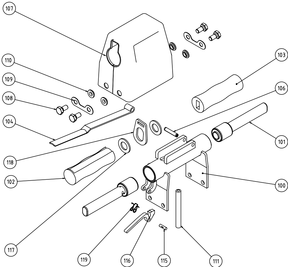
Figure 6-7. Handle Assembly
