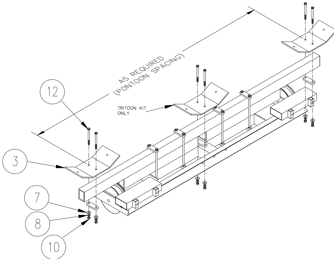
Figure 2. Mount Pontoon / Tritoon Cradles to Carriage
