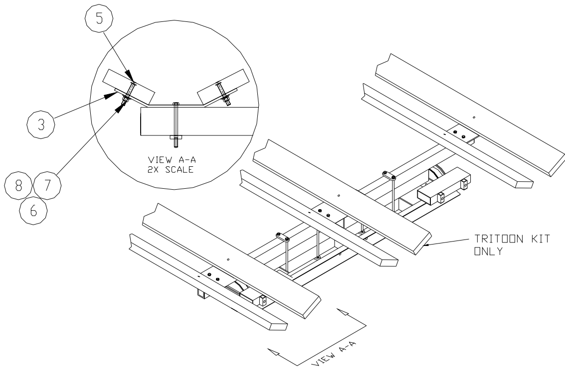
Figure 3. Mount Bunk to 4-Hole Support Plates
