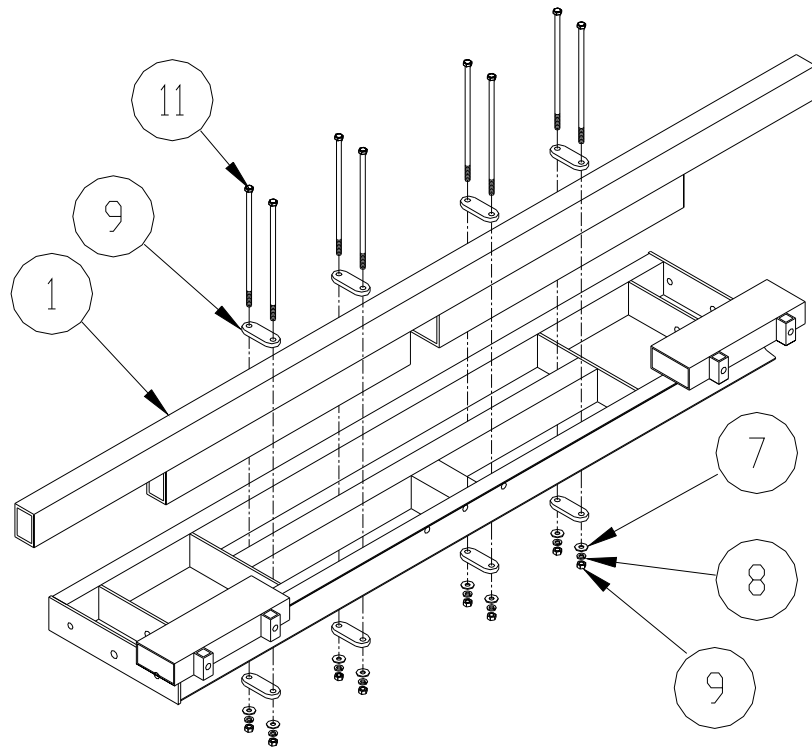
Figure 1. Cradle Support Weldment Assembly
