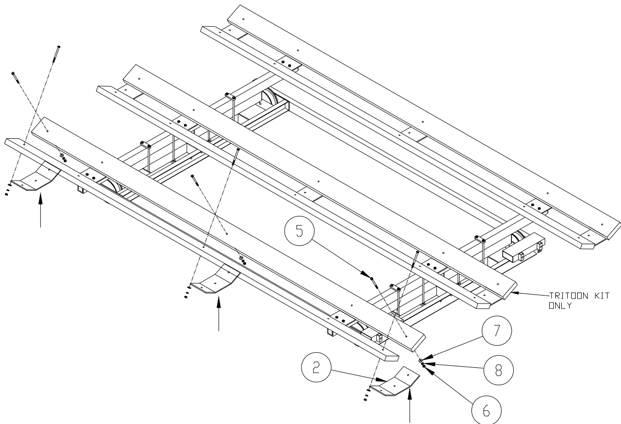
Figure 4. Mount Bunk Support Plates 3-Hole
