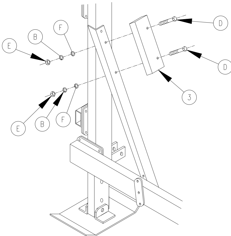
Figure 2-5. Lower Carpeted Wood Bumper
