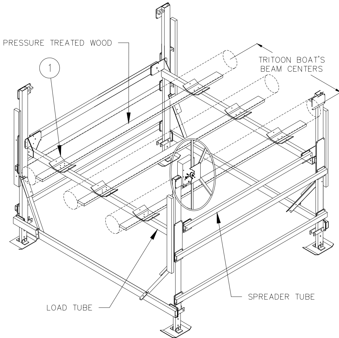
Figure 2-1. Cradle Positioning
