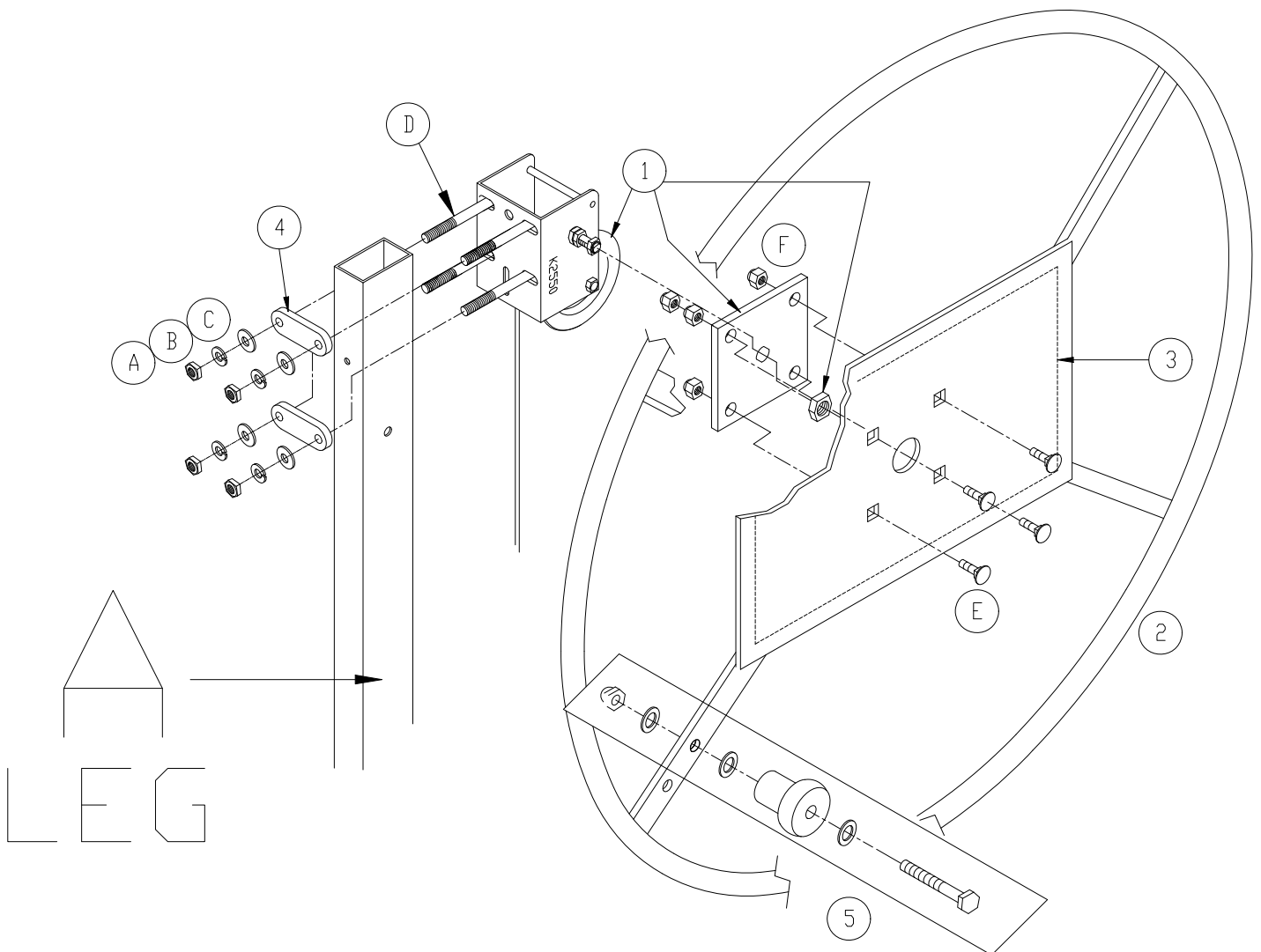
Figure 1 Mounting of Winch to Lift
