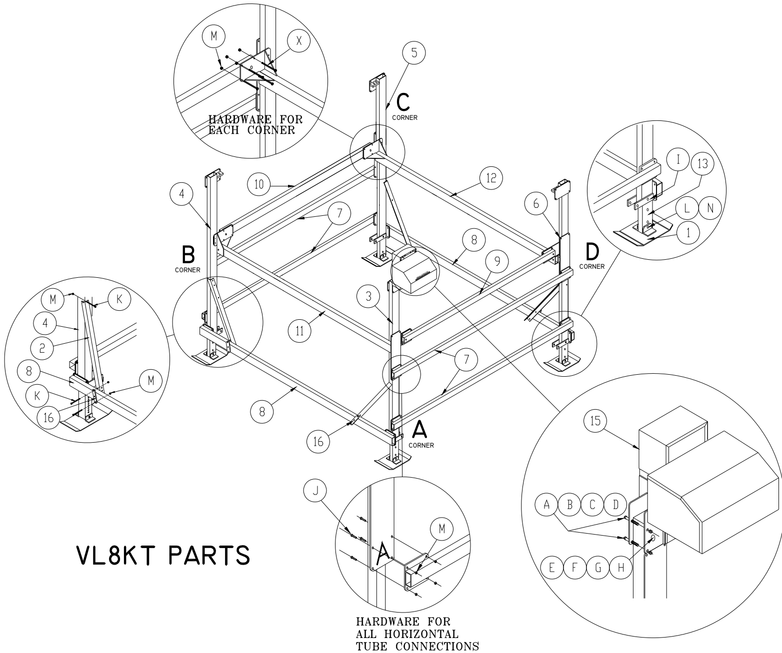
Complete VL 8KT Lift Assembly
