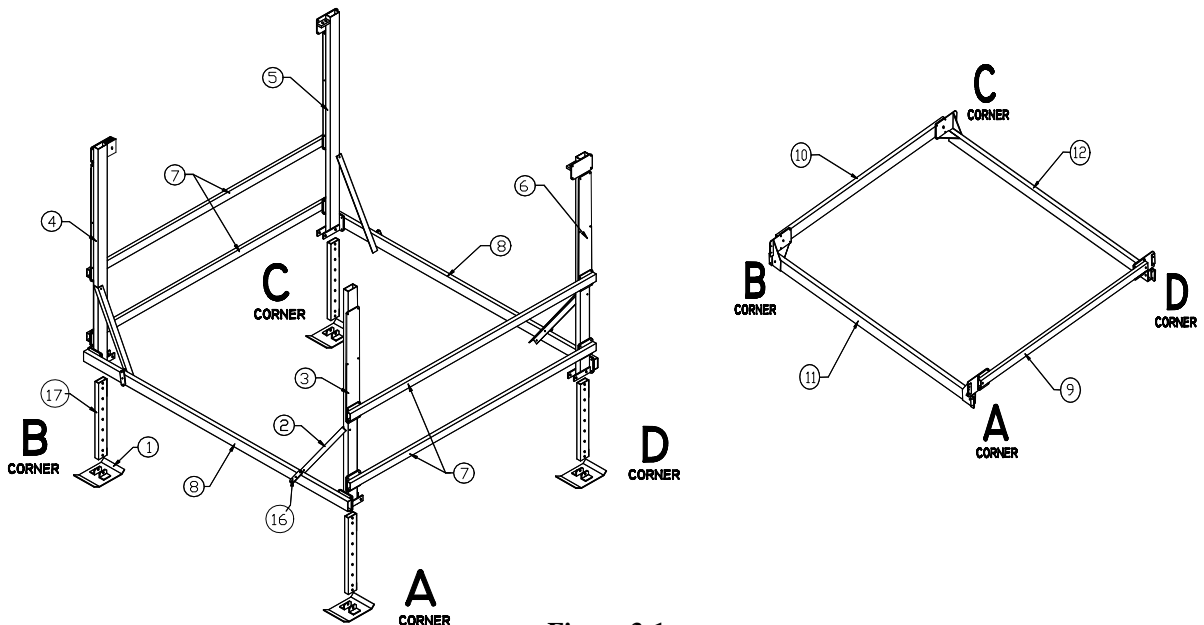
Figure 3-1. Vertical Lift Frame & Platform Assembly
