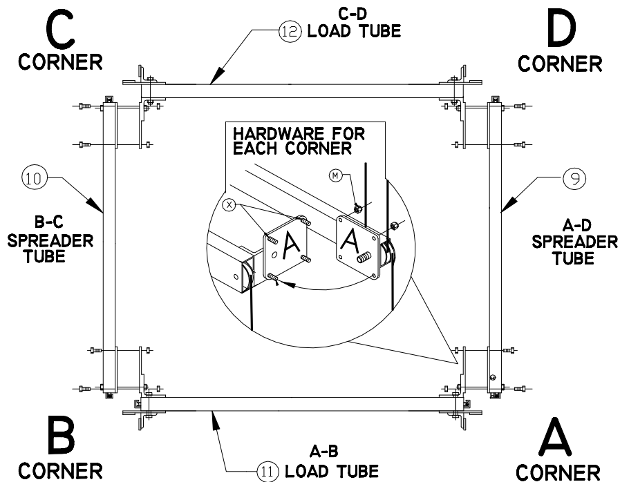
Figure 3-5. Platform Assembly – Top View
