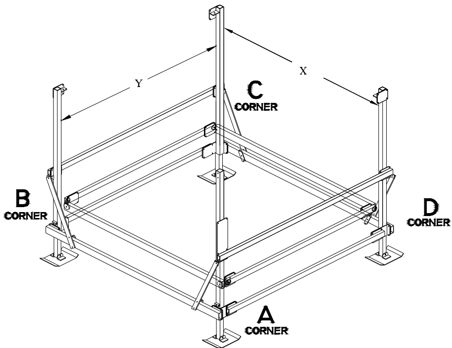
Figure 3-6. Frame Squaring Assembly / Table
